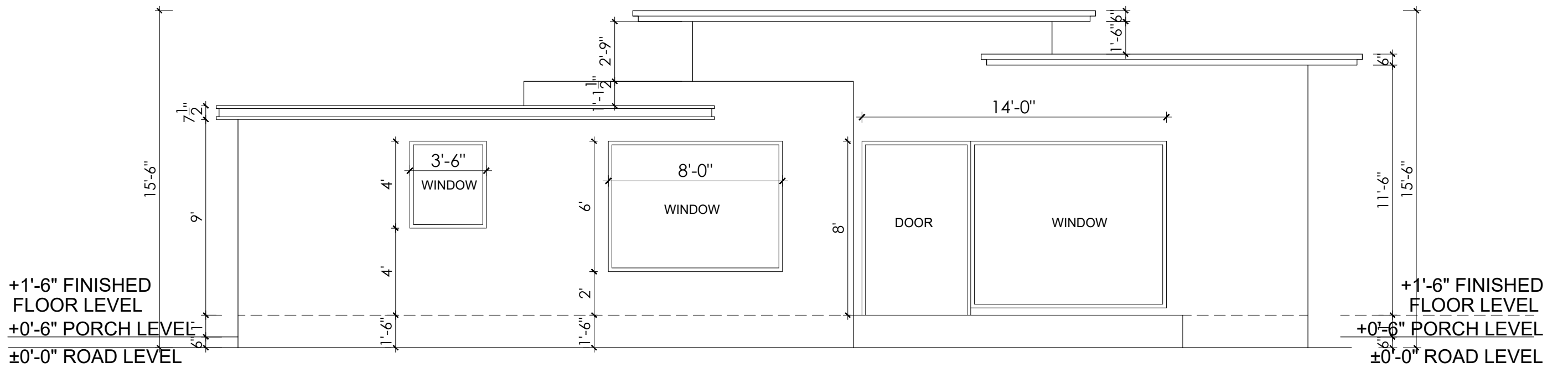
REAR ELEVATION
